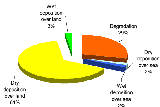
Fig. 1. Calculated annual balance of PCP removal from the atmosphere
