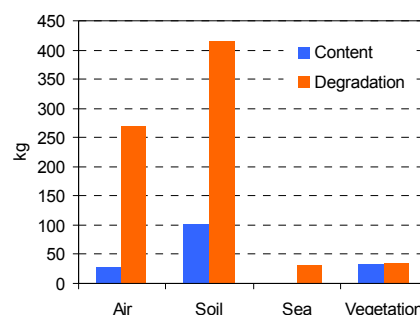
Fig. 4. Annual degradation and media balances for PCP
