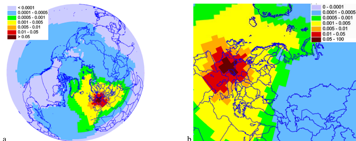
Fig. 2. Spatial distribution of pentachlorophenol concentrations in the above-ground air in the Northern Hemisphere (a) and in the EMEP domain (b), relative units
