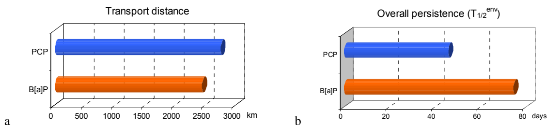
Fig. 5. Transport distance and Half-life in the environment calculated for PCP and B[a]P
