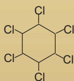
\gamma -HCH
